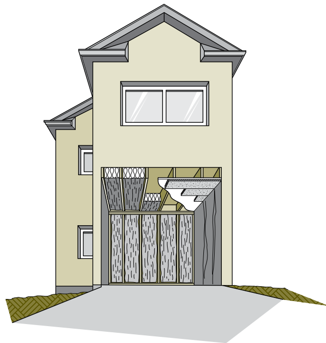
Figure 7-11 Air seal and insulate between an unheated garage and the house
